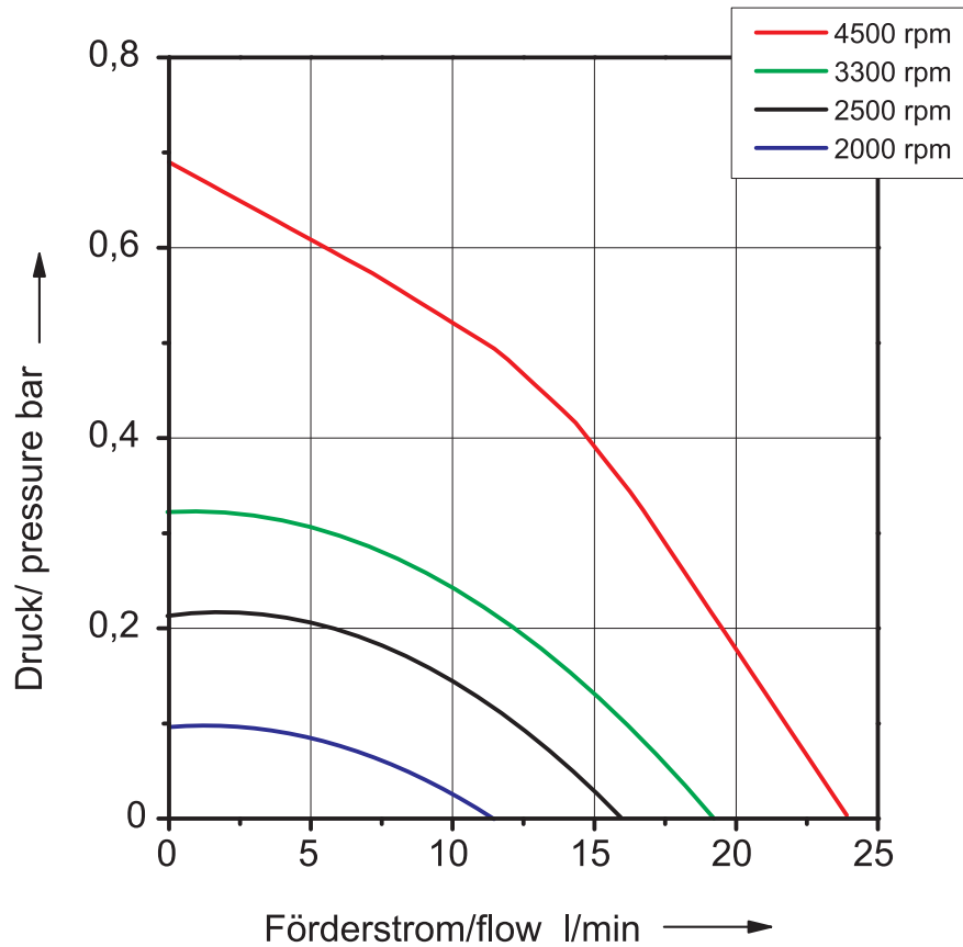
Pumpenkennlinie/ pump curve Ministat 125, 230, 240
